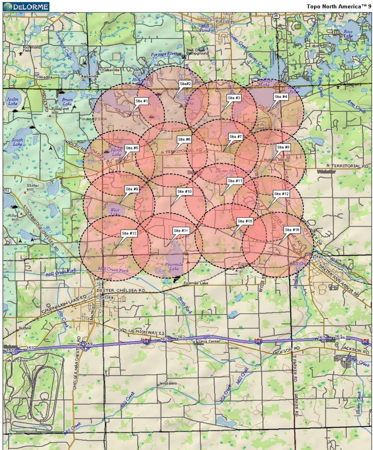
Map 3 - Siren Coverage Map (Whelen WPS 2900-10 at 70 db)
